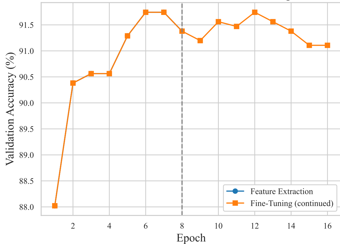
Plot 11: Feature Extraction vs. Fine-Tuning
